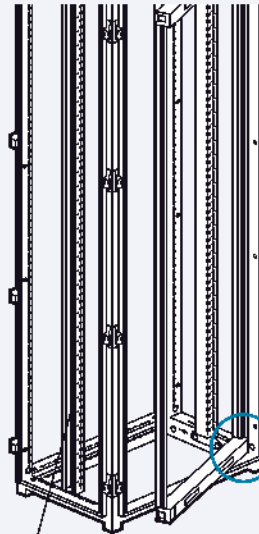
with reduced functional upright Cat.No 0 205 12
