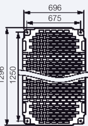
Lina 25 perforated plate Cat.No 0 346 09
